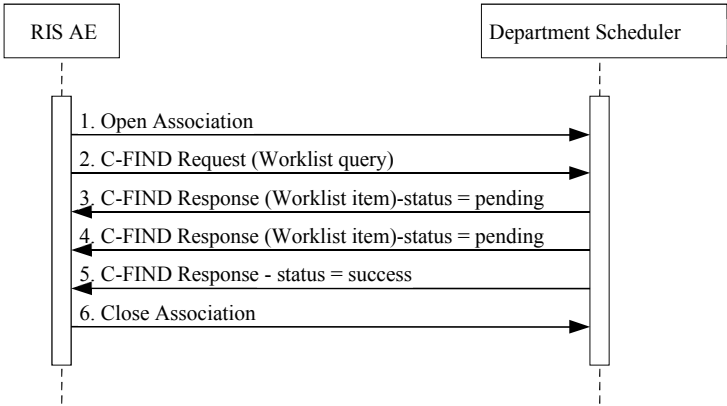
Figure 2.2-4: Sample Sequencing Diagram for Refresh Worklist
